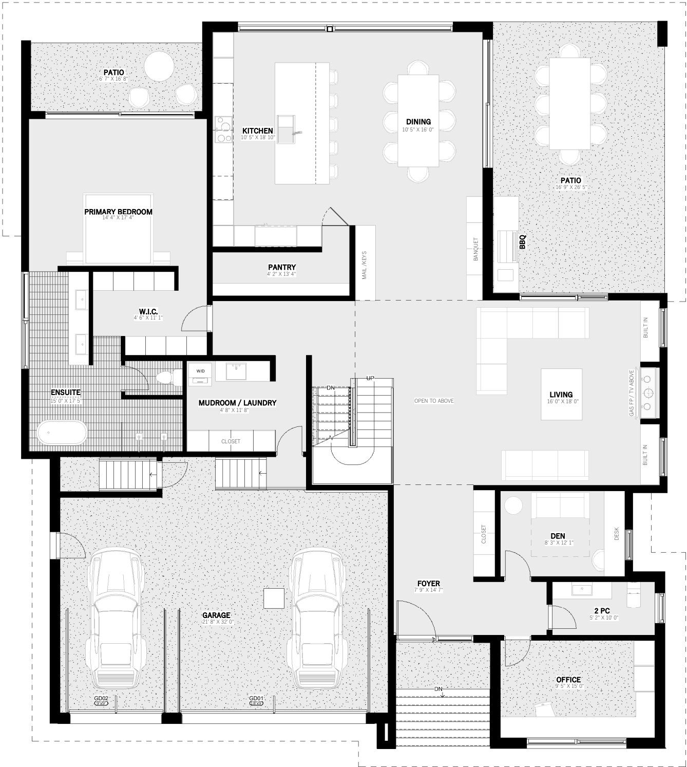
1st LEVEL- HOUSE LOT 20
